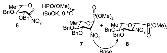
Scheme 3. Michael-type addition of \text{HPO}(\text{OMe})_2 to 2-nitrorhamnal 6
